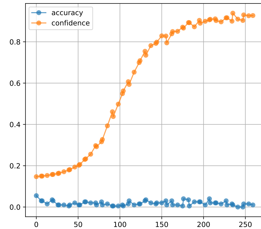
Evaluation Metrics
